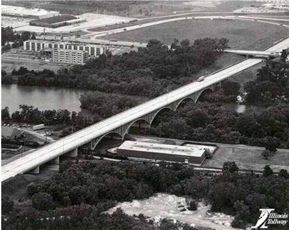
Aerial view of the Fox River Bridge on the Reagan Memorial Tollway (I-88), circa 1960. It is the only arched bridge in the Tollway system. All photos: Illinois Tollway.
