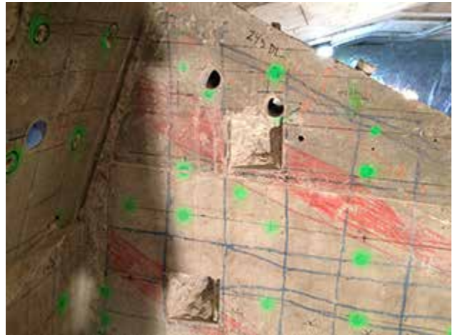
Coring layout at pier diaphragm and hand chipping to visually identify tendon location.
