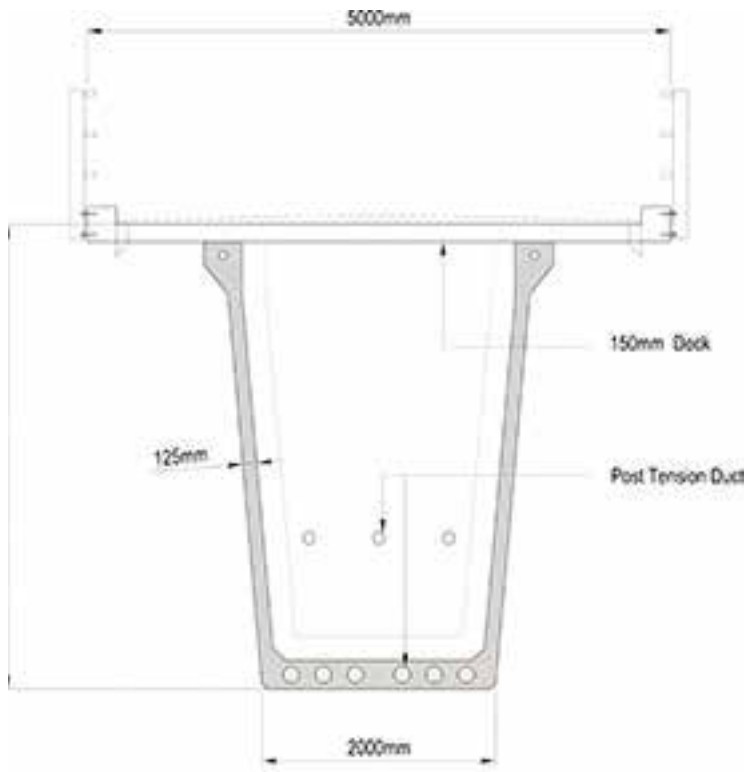
Typical Section at Midspan
