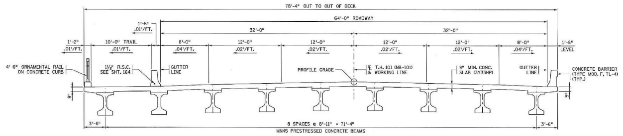
TRANSVERSE SECTION
