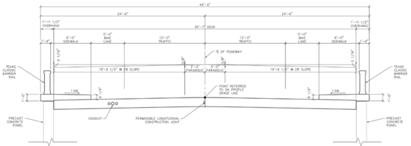
RHOMBERG AVENUE BRIDGE TYPICAL SECTION LOOKING UPSTATION
