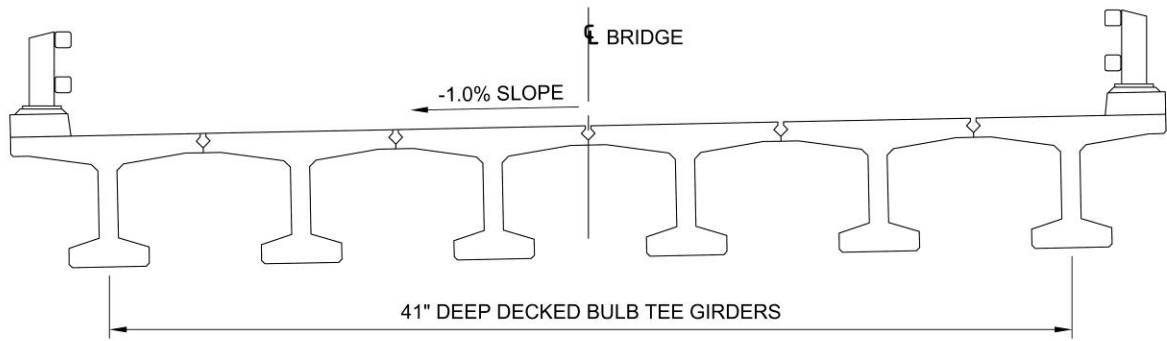
TYPICAL BRIDGE SECTION
